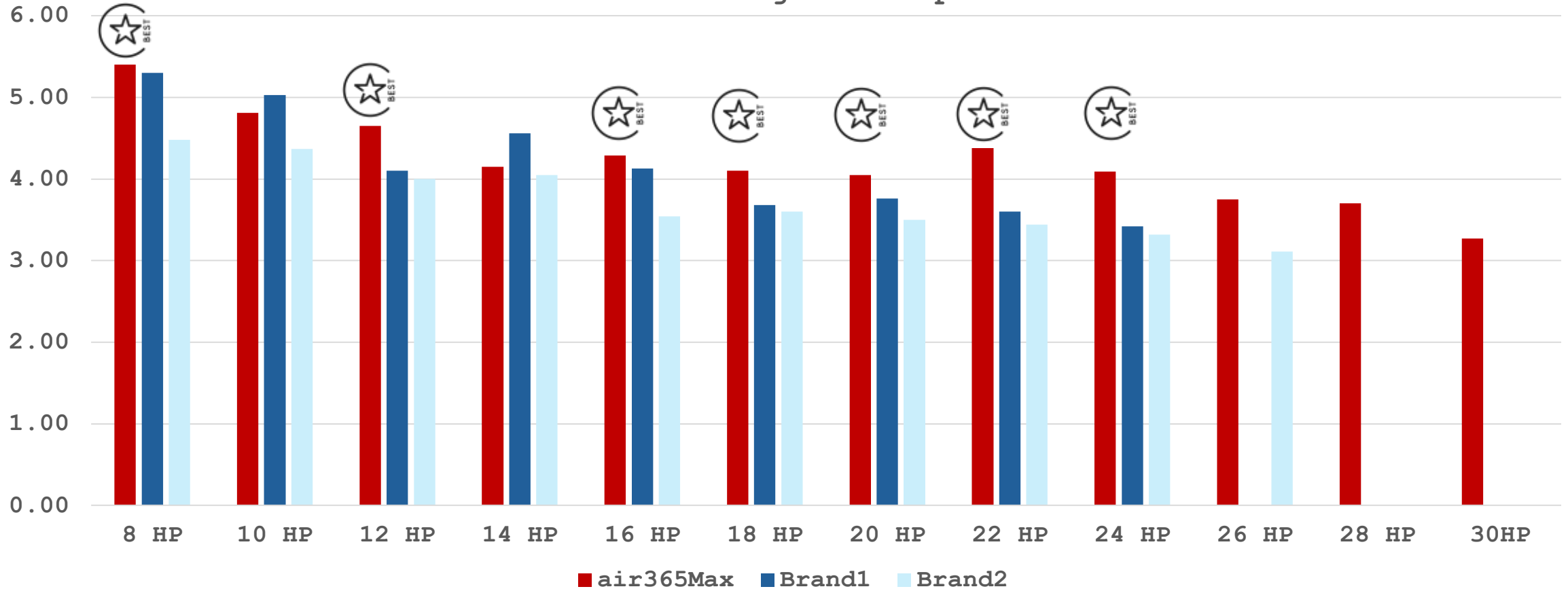
Cooling COP Comparison
